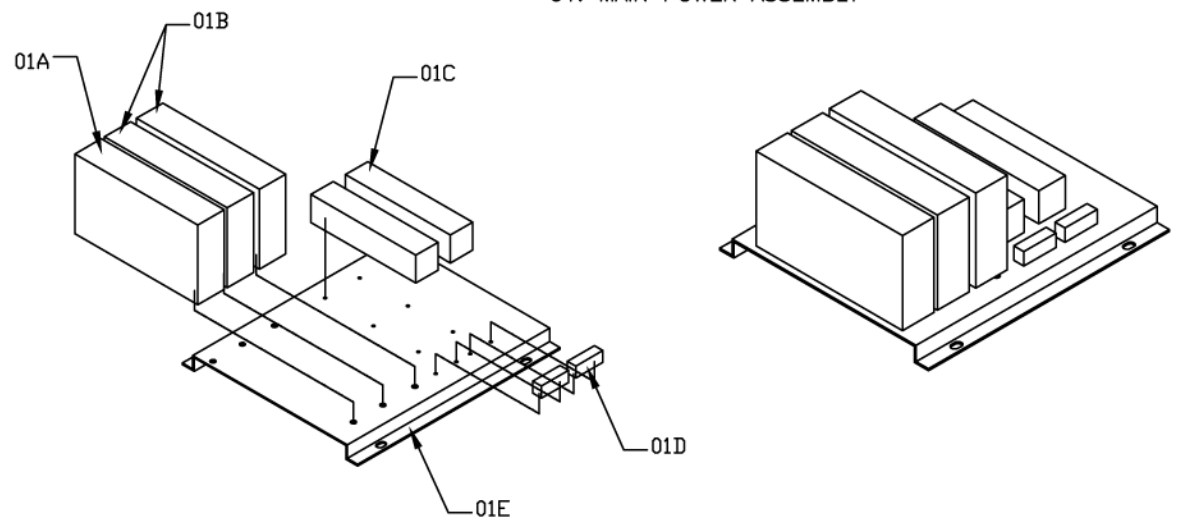
01. MAIN POWER ASSEMBLY
