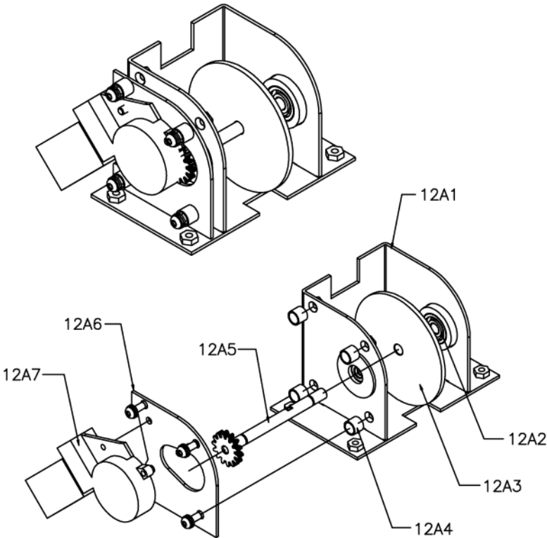
12A. LHG A006A DRIVEN MECHANISM ASSEMBLY
