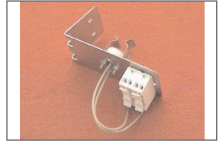
2640.0020 Halogen spot Giga without plate/lamp
